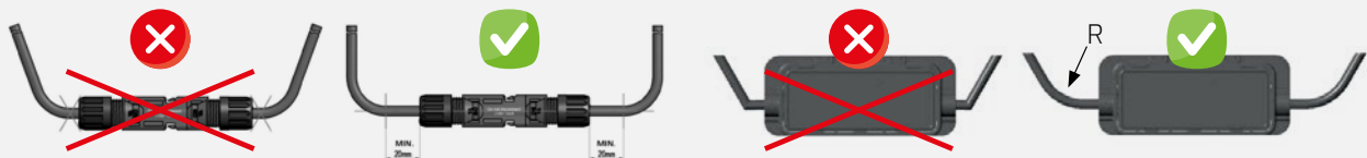
Fig. 5: permissible bending radius of the solar cables
