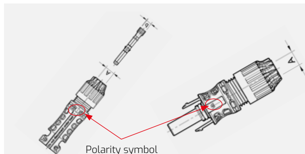
Fig. 7: Indication of polarity of the MC4-Evo2 connectors
